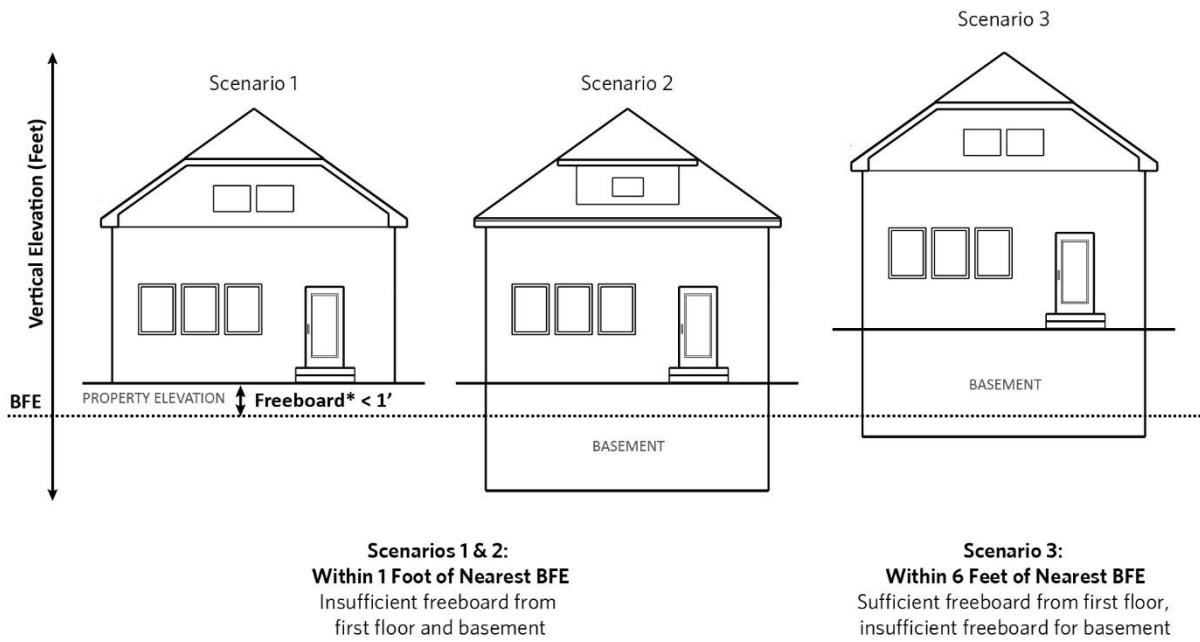
Figure 9. Diagram of development near the base flood elevation (BFE)
