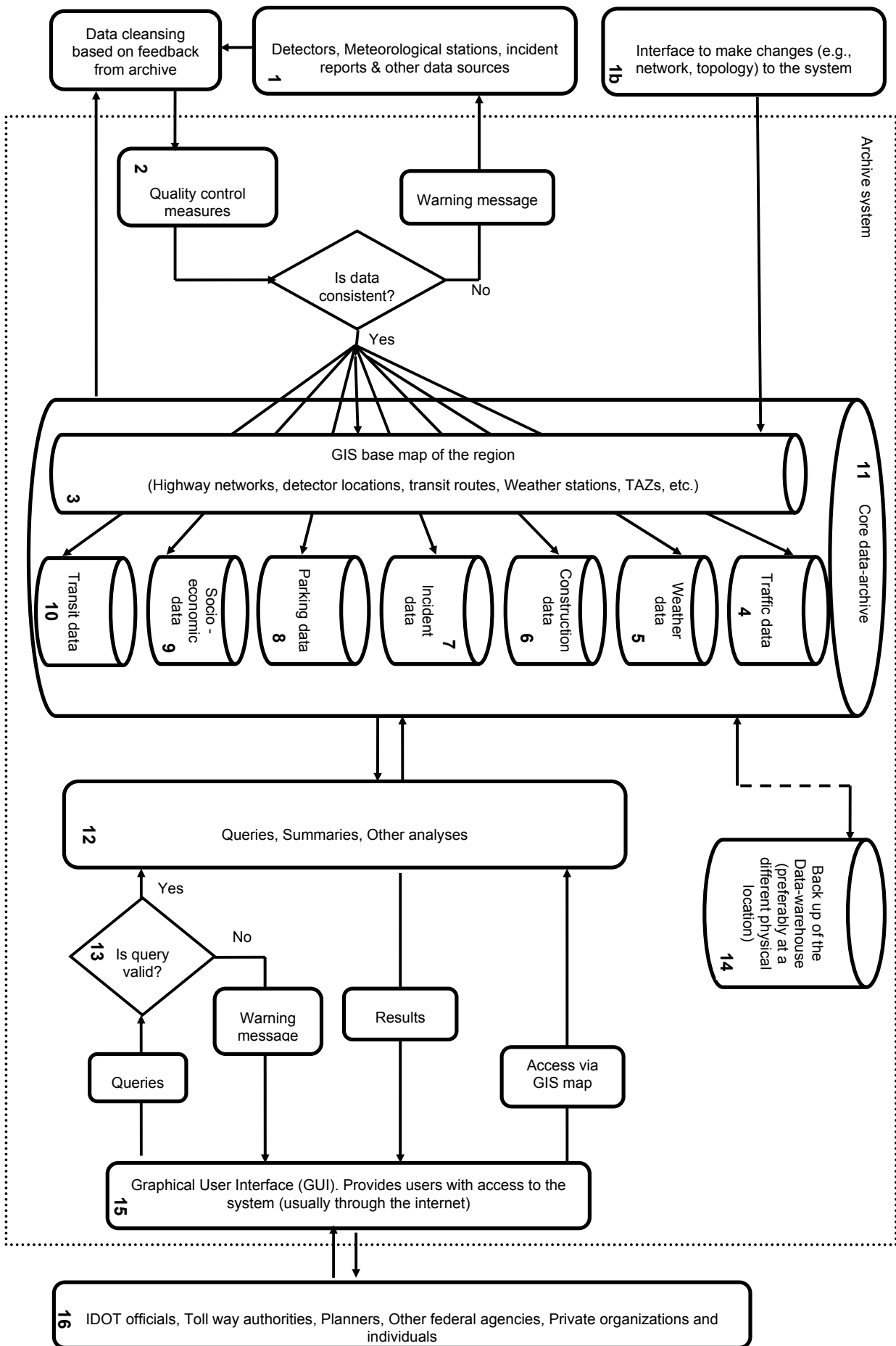
Figure 4-1: Conceptual Schematic of the Regional Data Archive System
