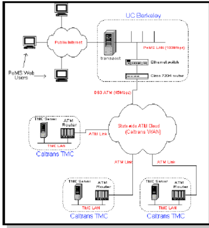
Figure 2-2: High-Level Communication Architecture of PeMS
