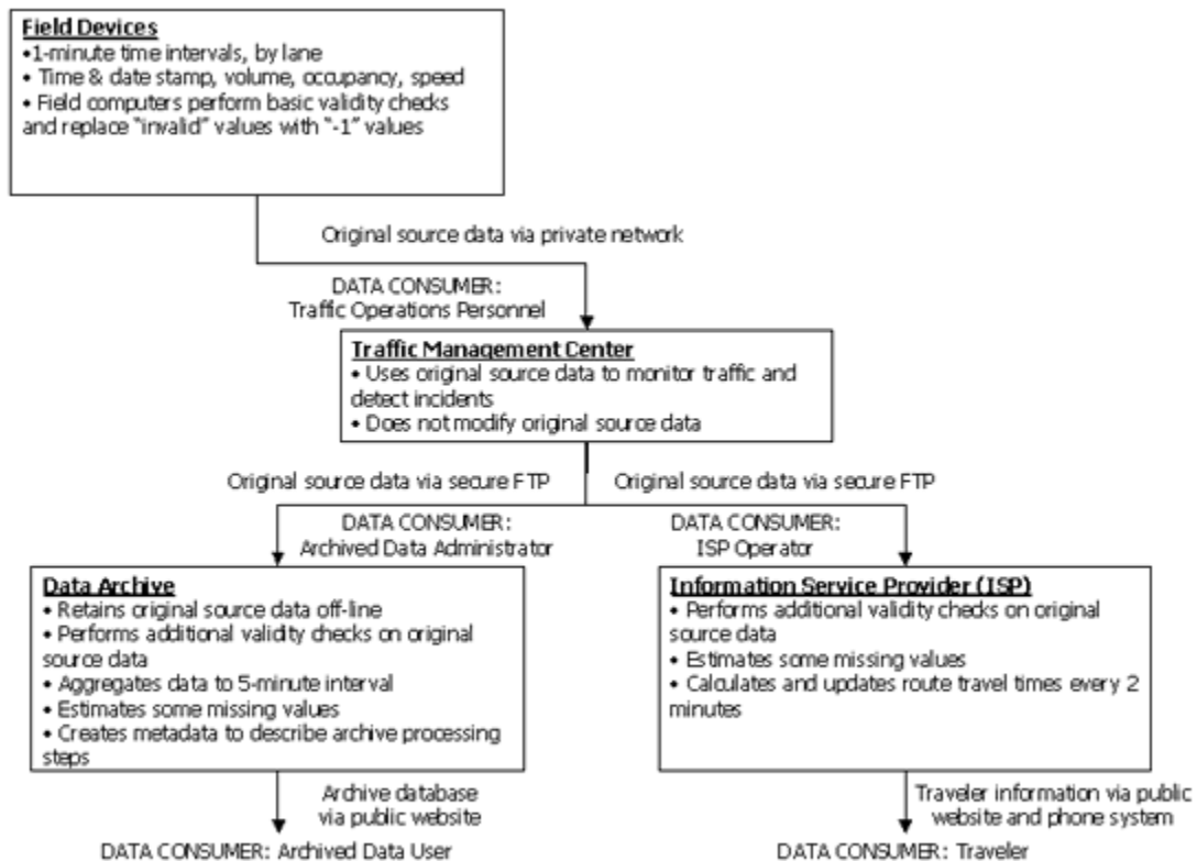
Figure 2-1: Data Flows and Data Consumers in Austin Case Study
